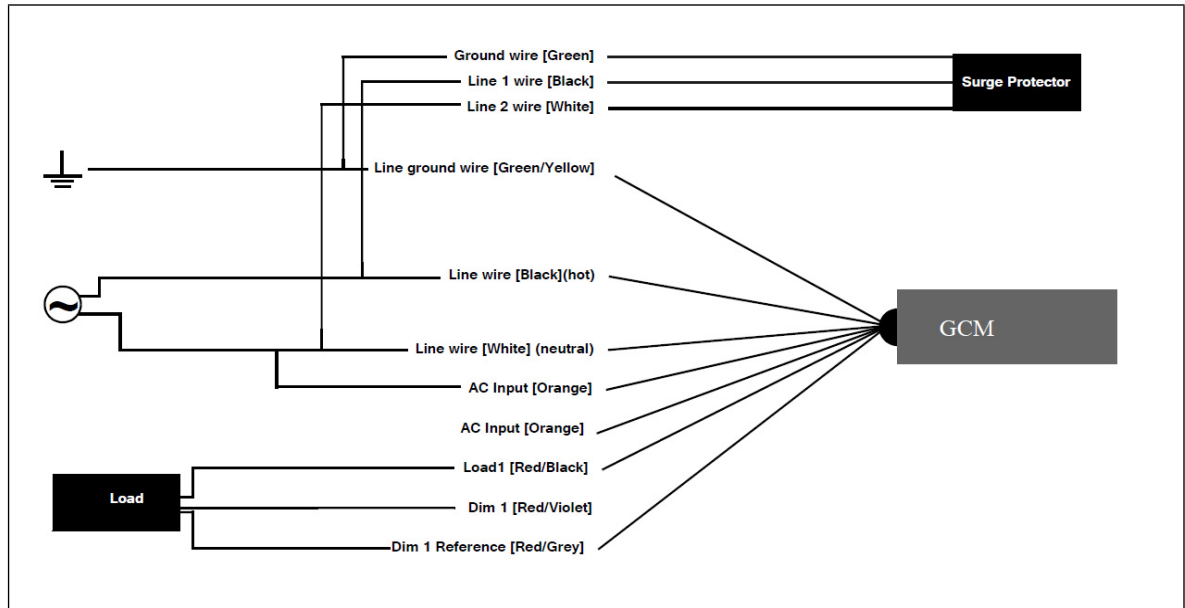
Figure 1: GCM Wiring Guide
