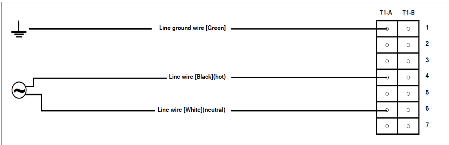
Figure 1: POV Wiring Guide
